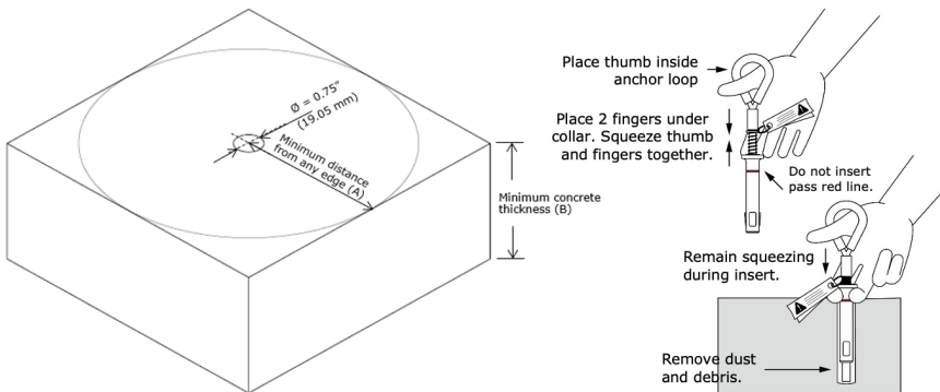
Figure 5 - Hole Drilling Instructions
